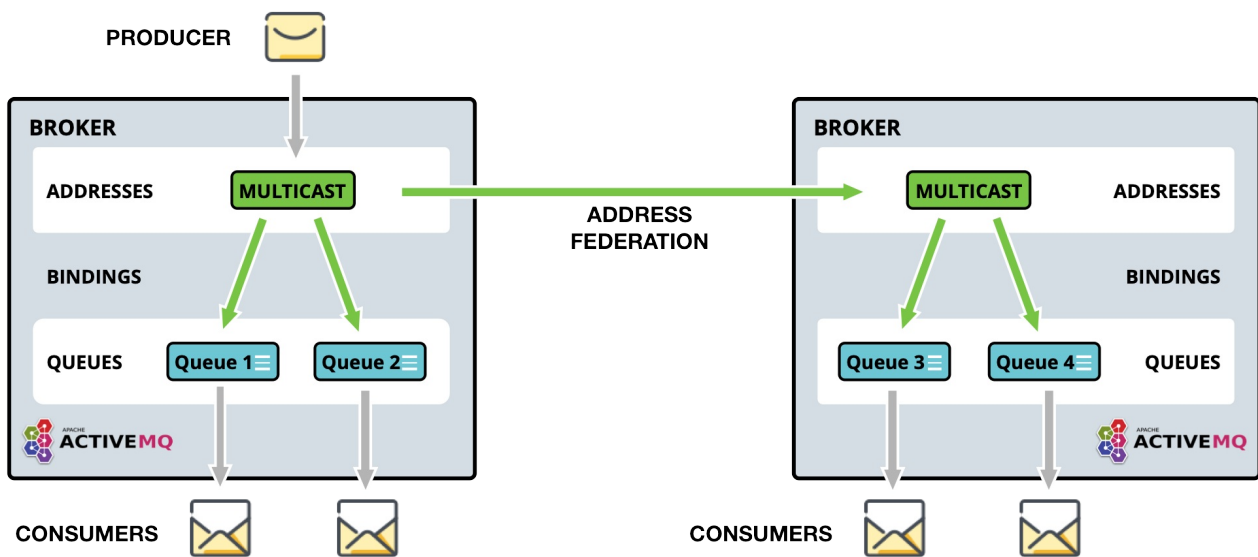
Figure 1. Address Federation
