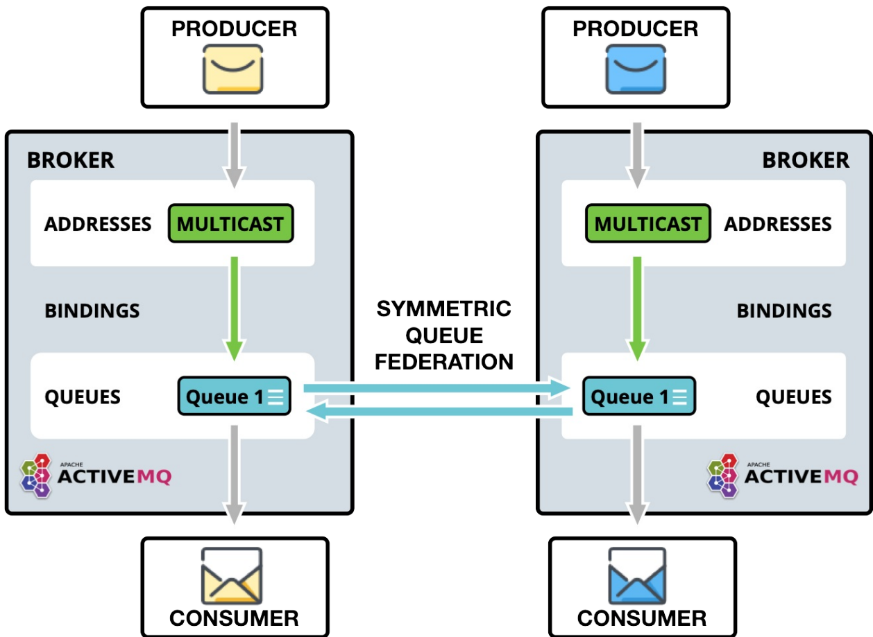
Figure 2. Queue Federation
