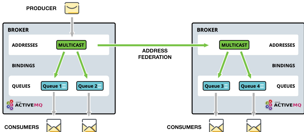
Figure 1. Address Federation
