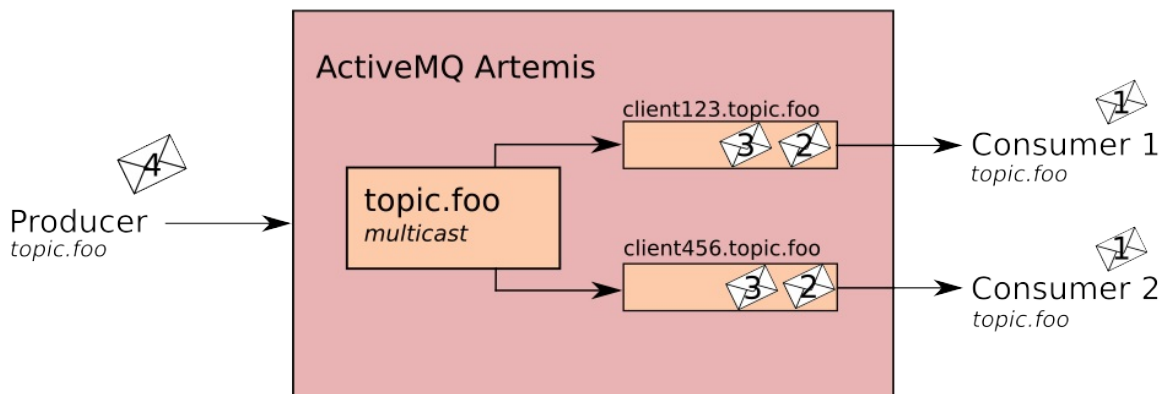
Figure 2. Publish-Subscribe
